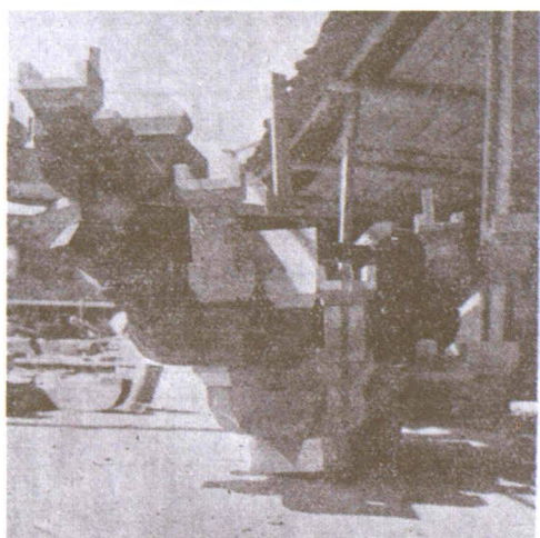
轩平基斗拱
